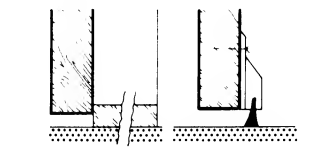
⑧ Draught excluders for old doors
